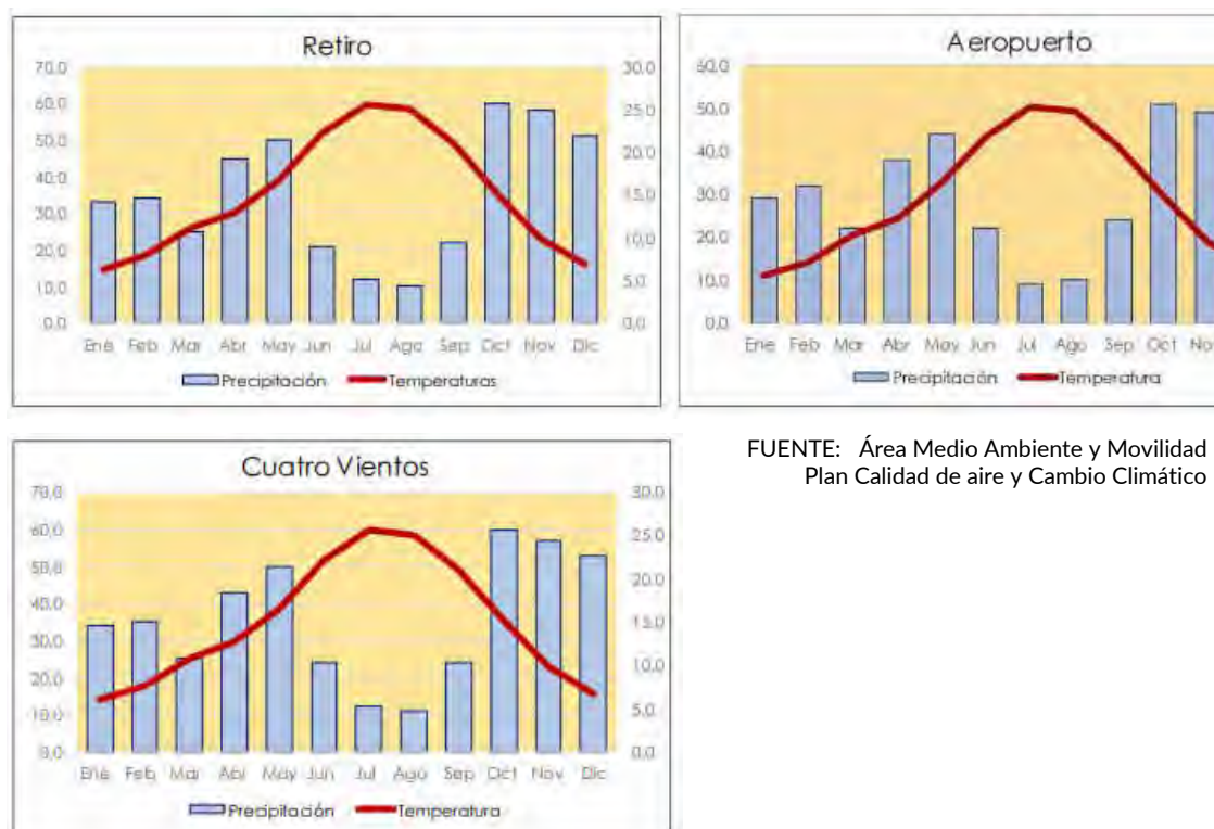
Fig. 22 Climogramas Observatorios Madrid
