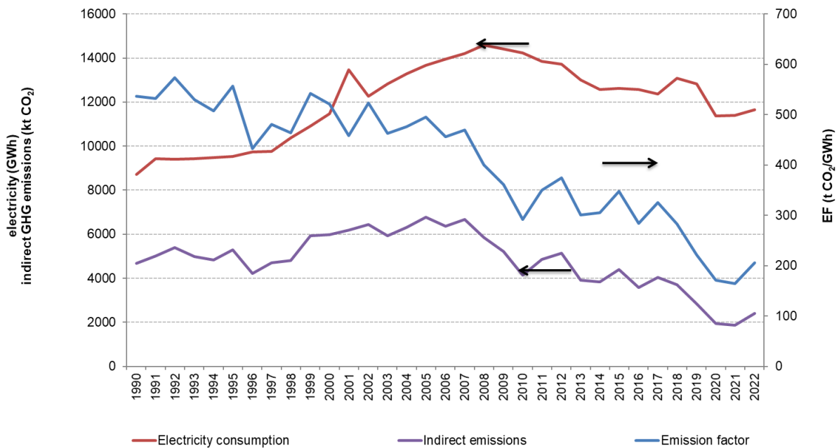
Figure 3. Evolution of indirect emissions (Scope 2+3), electricity consumption and electricity EF
