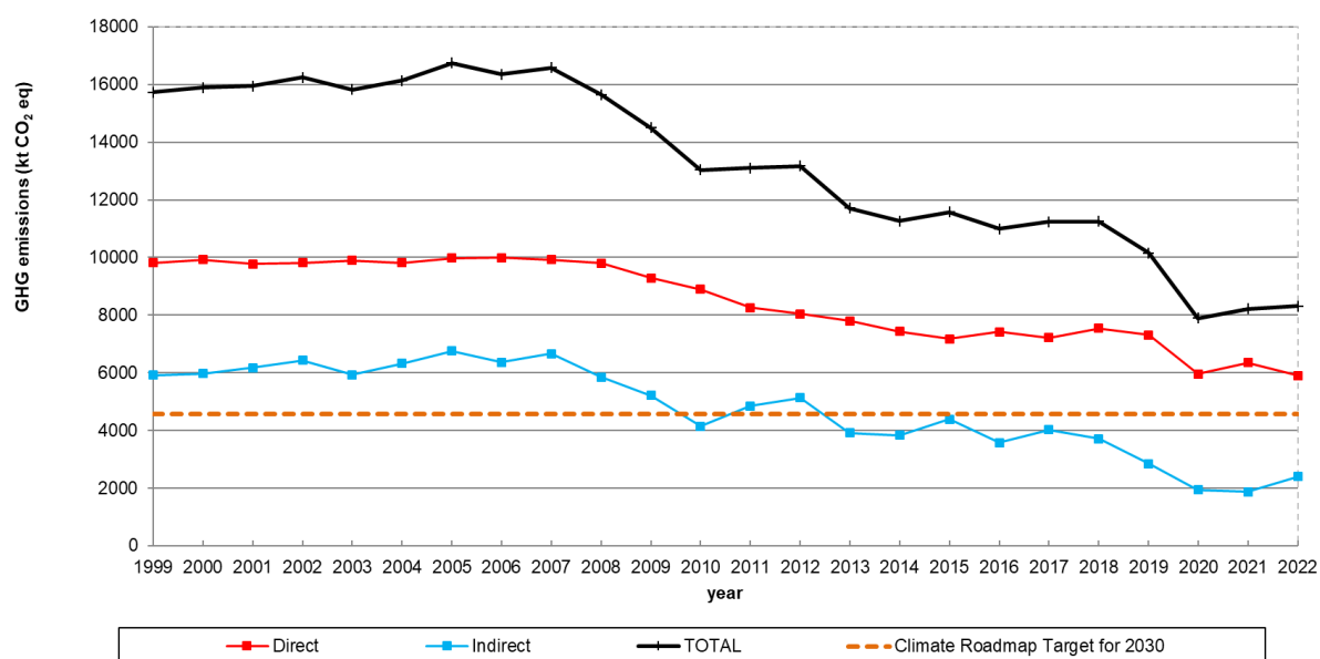
Figure 1. Scope 1 emissions trend by compound
