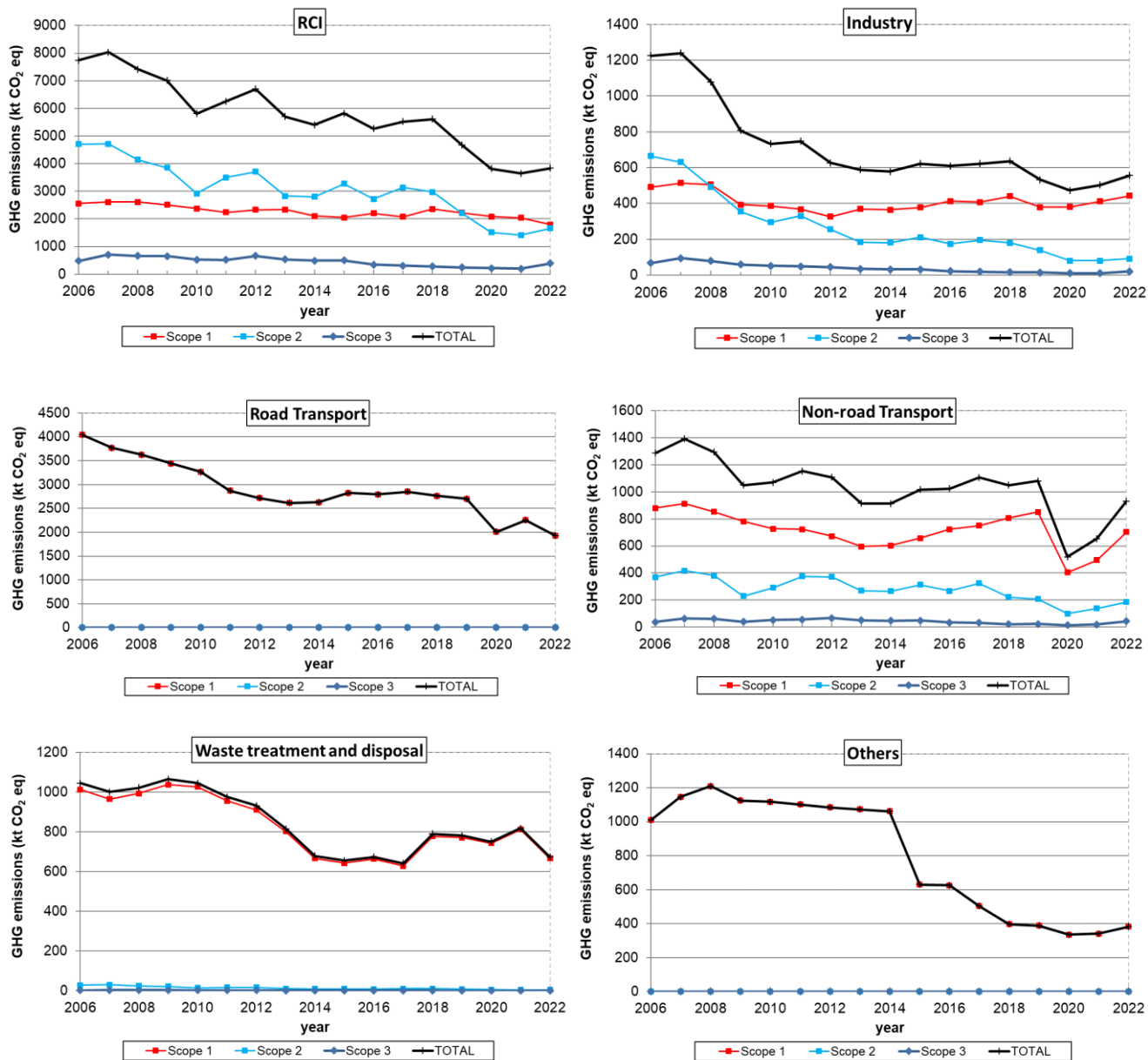
Figure 6. GHG emissions by scope and sector
