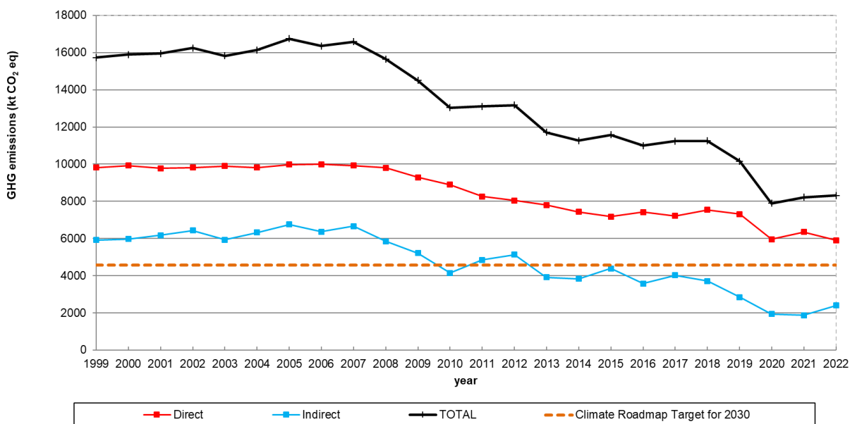
Figure 5. GHG emissions trends in Madrid city
